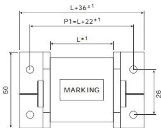
Outline drawing C...
